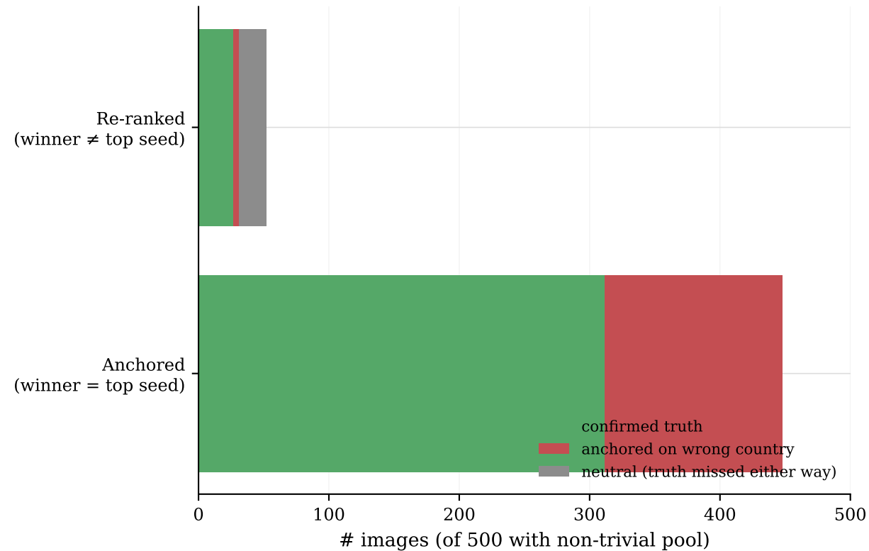
Anchoring outcomes
